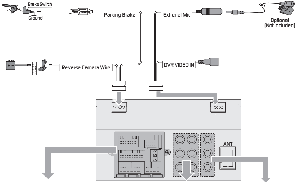
Connector C
